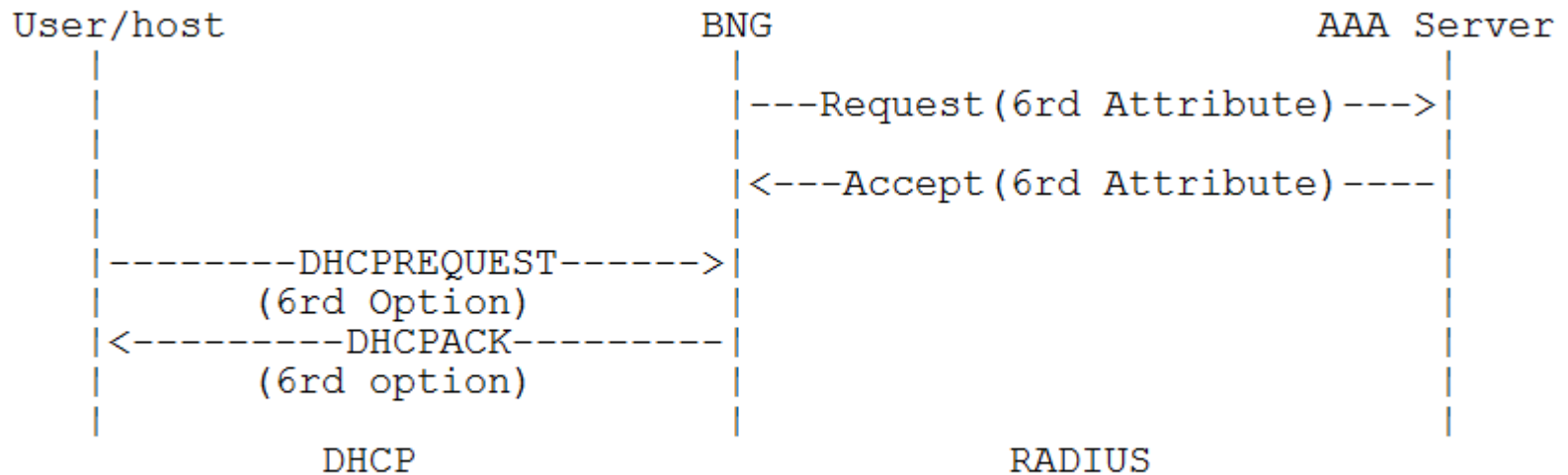
Figure 2: the cooperation between DHCP and RADIUS
