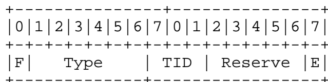
The Structure of the EVC NAL Unit Header
