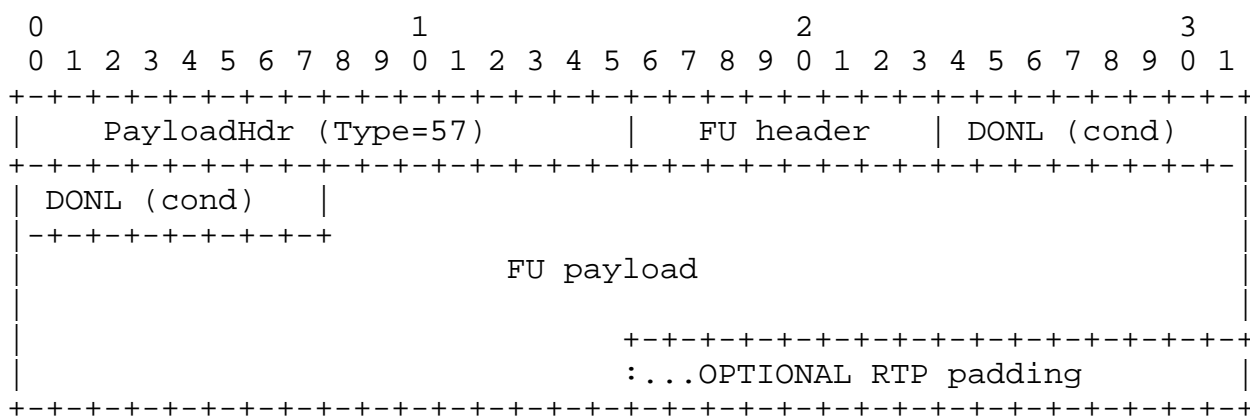
The Structure of an FU
