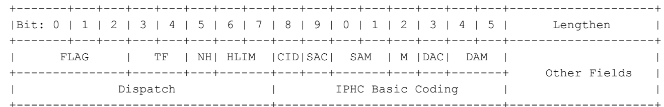
Figure 15: Internet Layer Header Common Format
