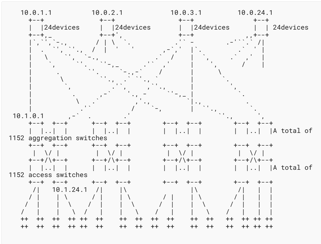
Figure 9: 48 pods, each of which has 24 aggregation switches and 24 access switches
