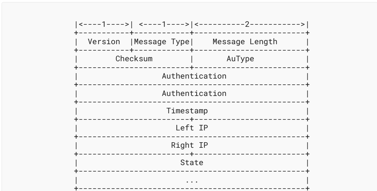
Figure 5: The Format of LFA Messages
