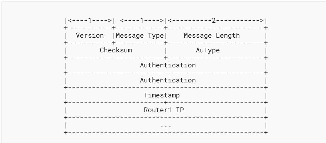
Figure 4: The Format of DA Messages
