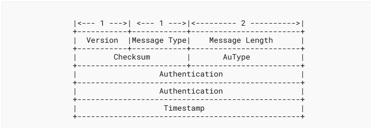
Figure 2: The format of FAR header
