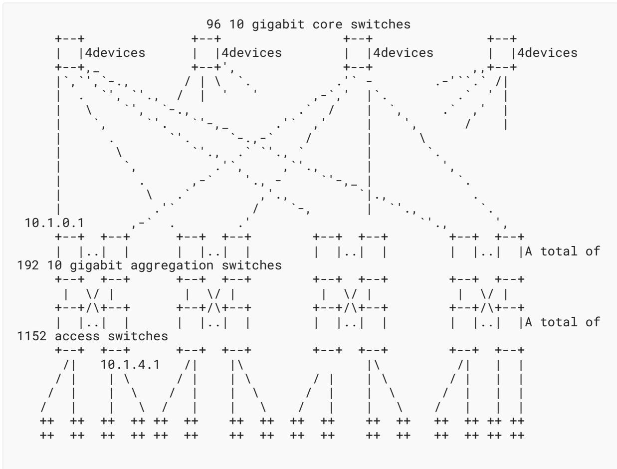
Figure 10: 48 pods. Each pod has 4 10G aggregation switches and 24 Gigabit access switches
