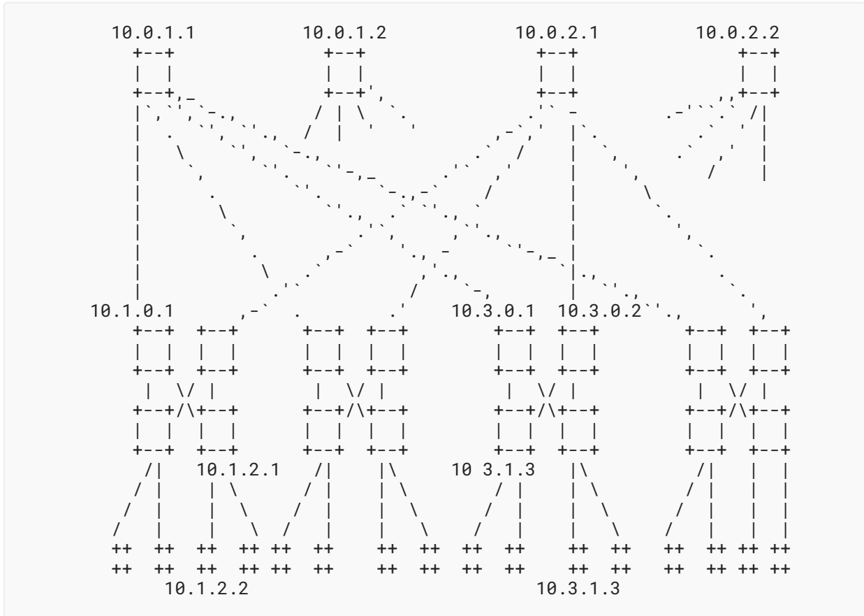
Figure 8: Fat-tree Network
