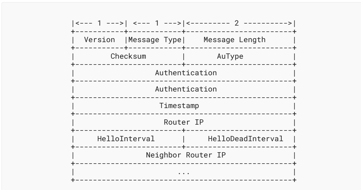
Figure 3: The Format of Hello Messages
