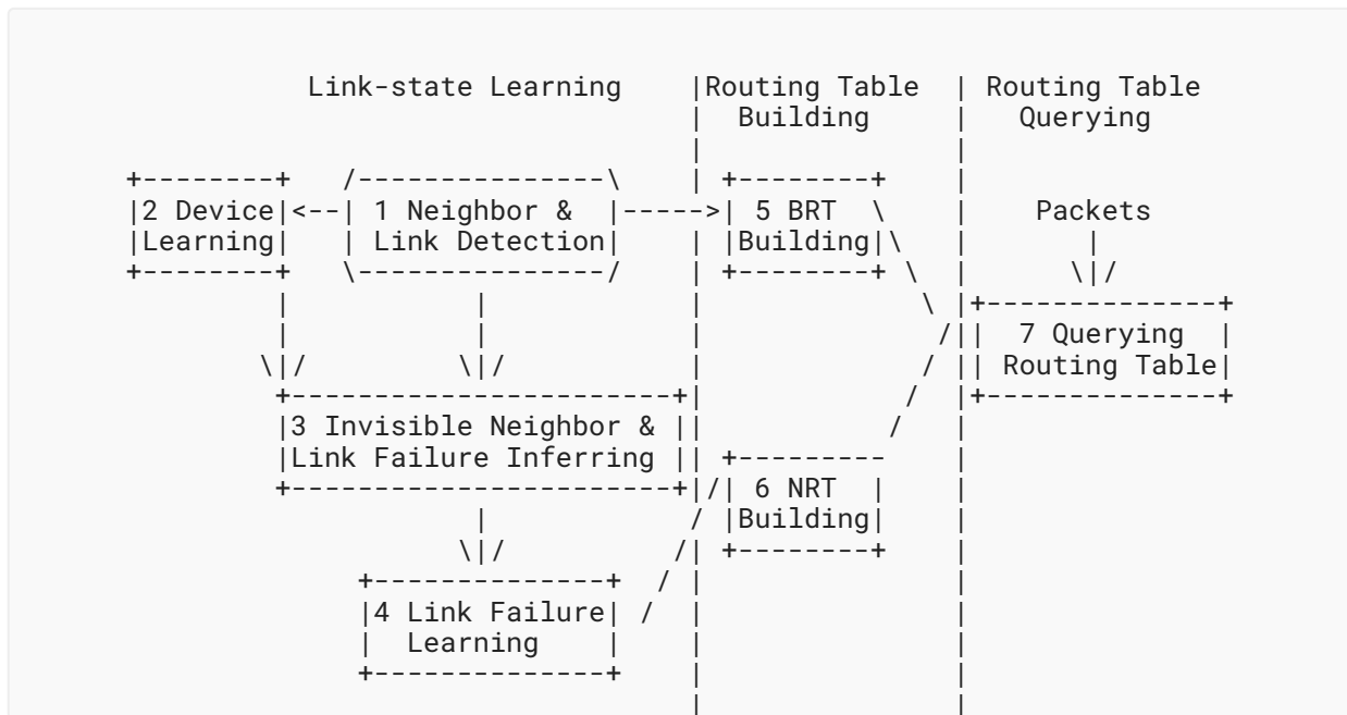
Figure 1: The FAR framework
