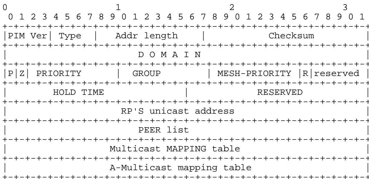
Figure 22 C-MAPPER/RP unicast HELLO/KEEP-ALIVE message to back up RPs
