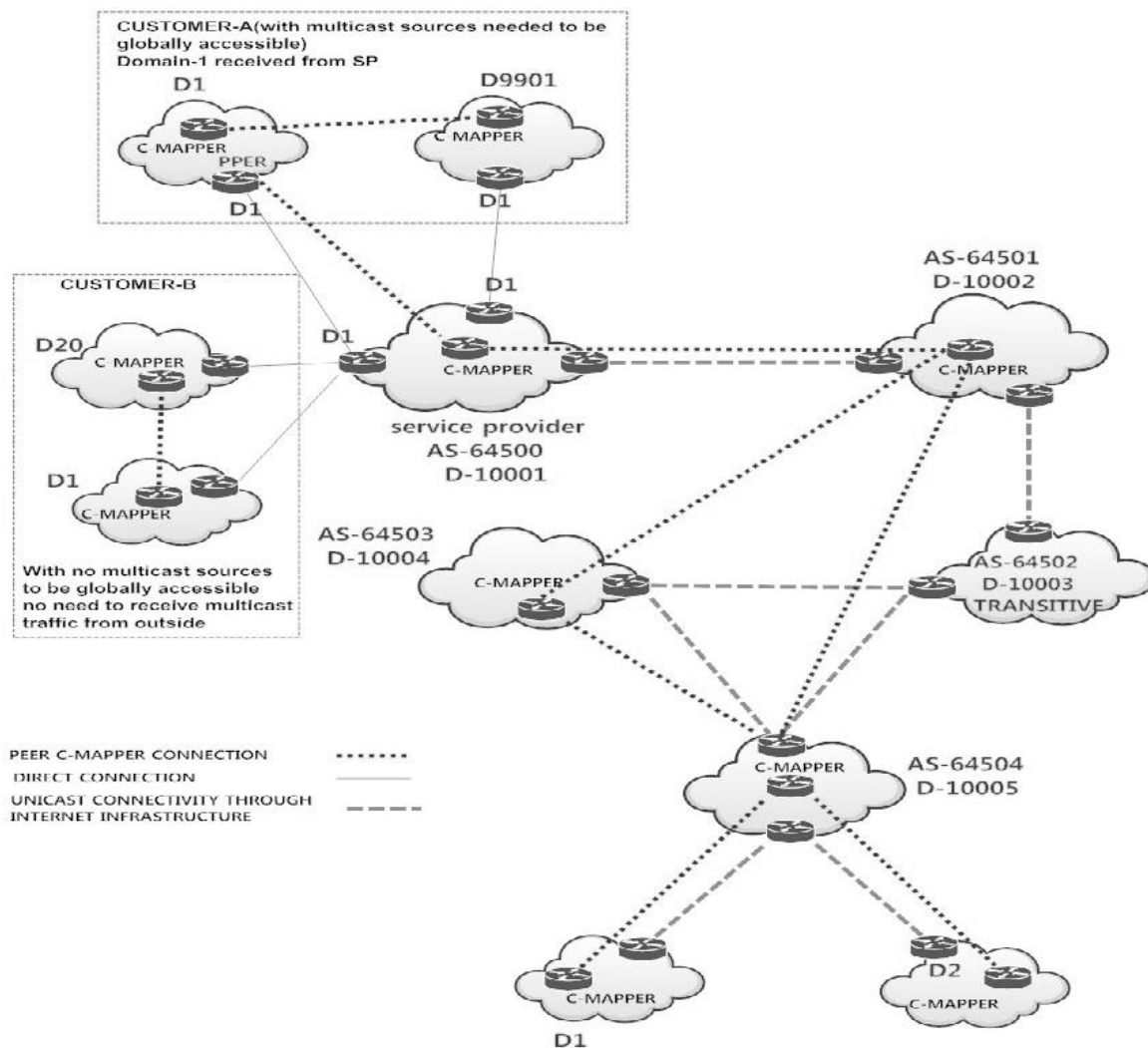
Figure 47 network with multiple multicast domains
