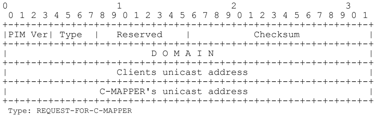
Figure 22 request- for-C-MAPPER packet sent to the SC-MAPPER
