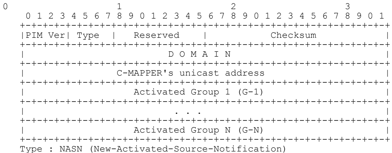
Figure 13 New-Activated-Source-Notification message format
