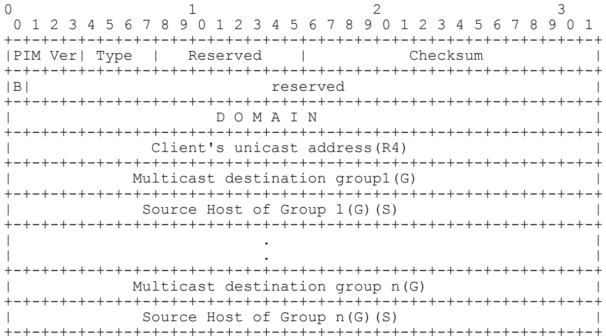
Figure 7 Client sends request to RP for a specific source
