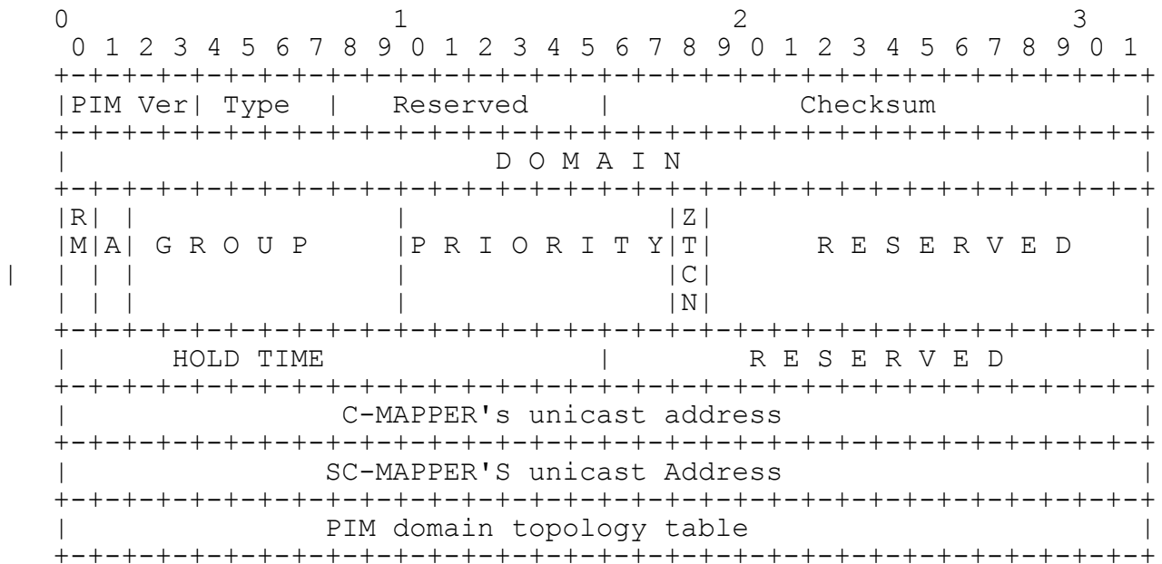
Figure 16 C-MAPPER-INTRODUCTION message sent to 239.0.1.190
