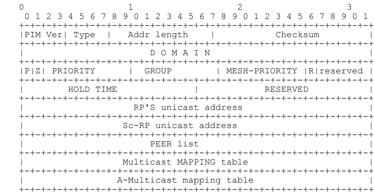
Figure 29 C-RP introduction message format
