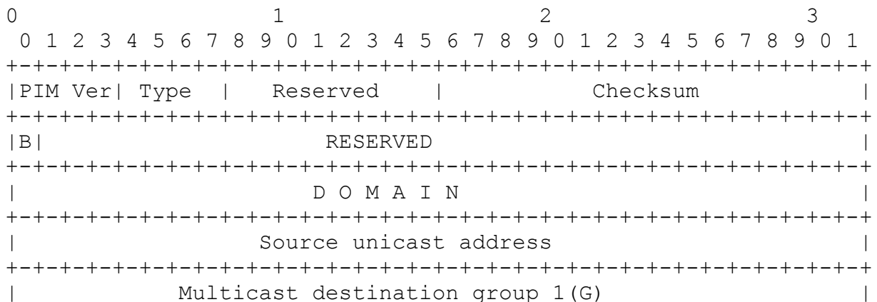
Figure 2 source register request packet
