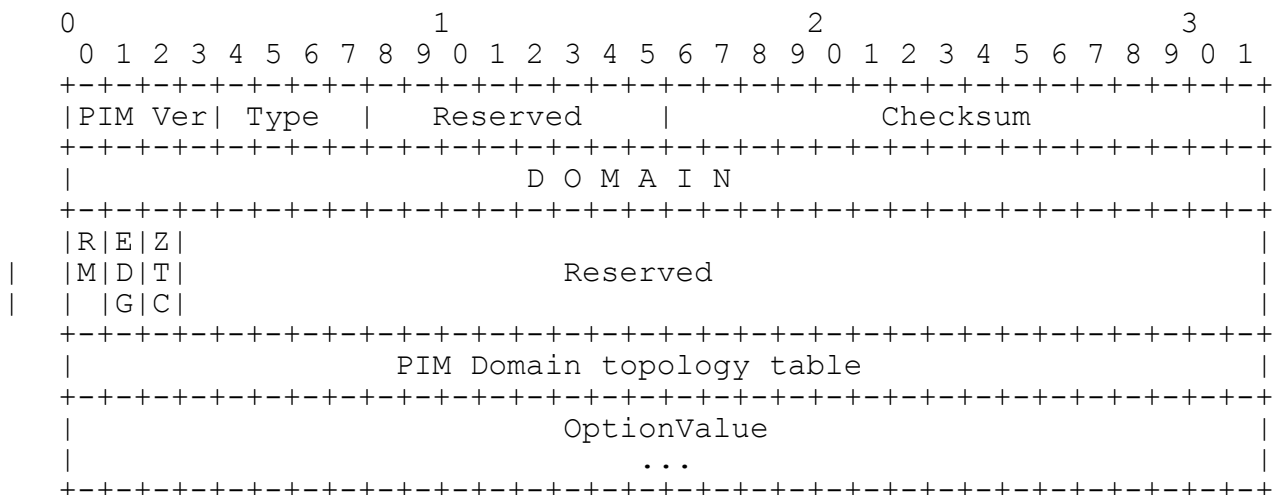
Figure 23 hello packet containing RP address
