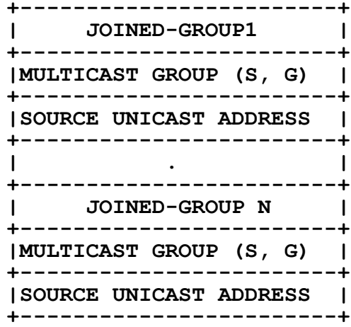
Figure 42 Joined-Groups table used by both TR'(s) and Clients
