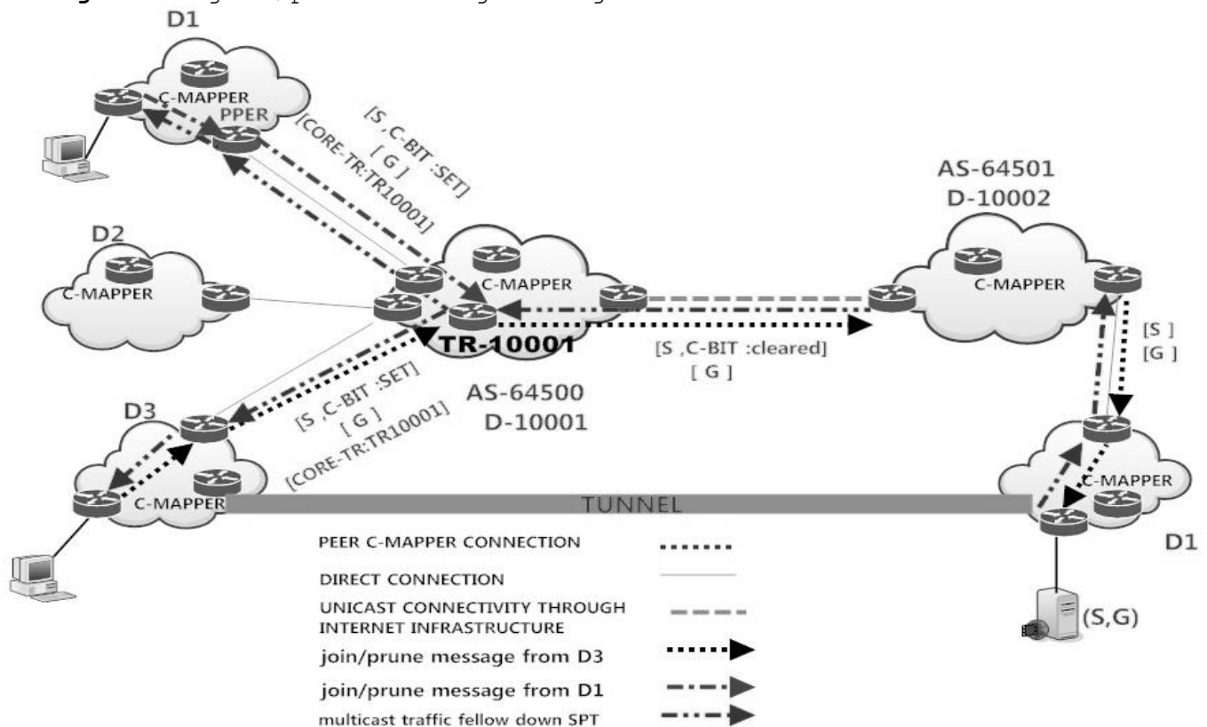
Figure 46 join/prune message being sent towards the source
