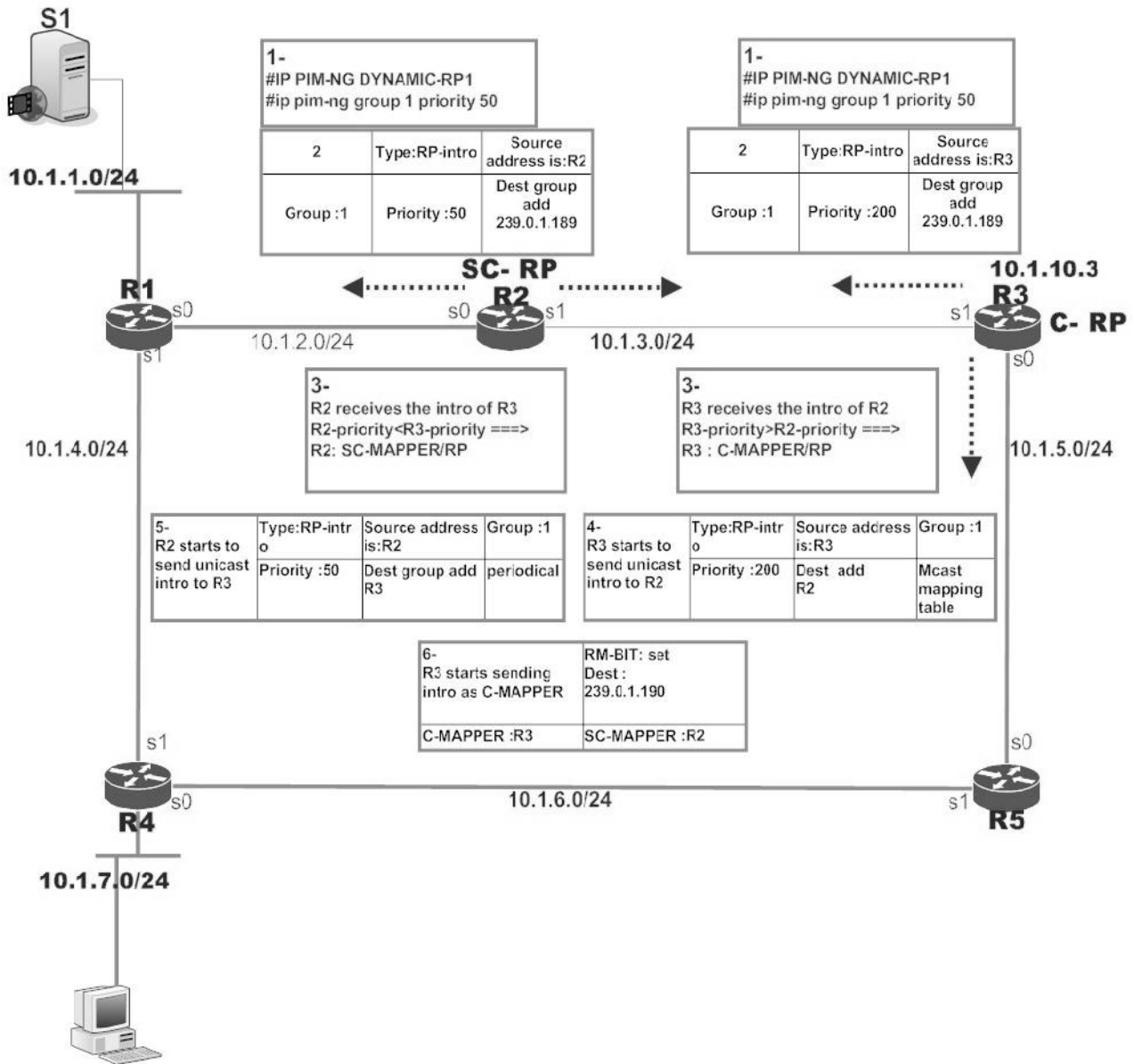
Figure 19 PIM-NG network with backup RP (SC-RP)
