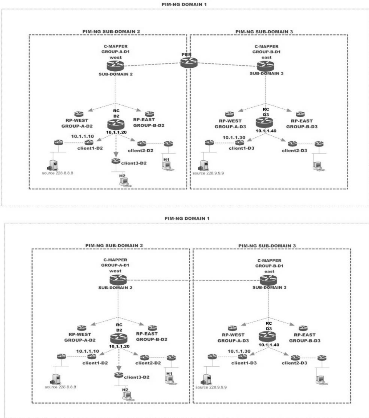
Figure 51 Sample PIM-NG domain Divided to Sub-Domains
