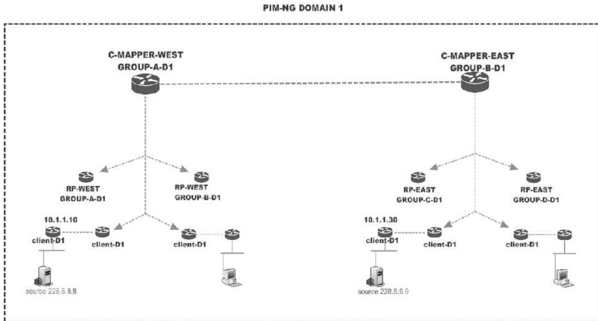
Figure 32 network with single multicast domain and redundant C-MAPPERS
