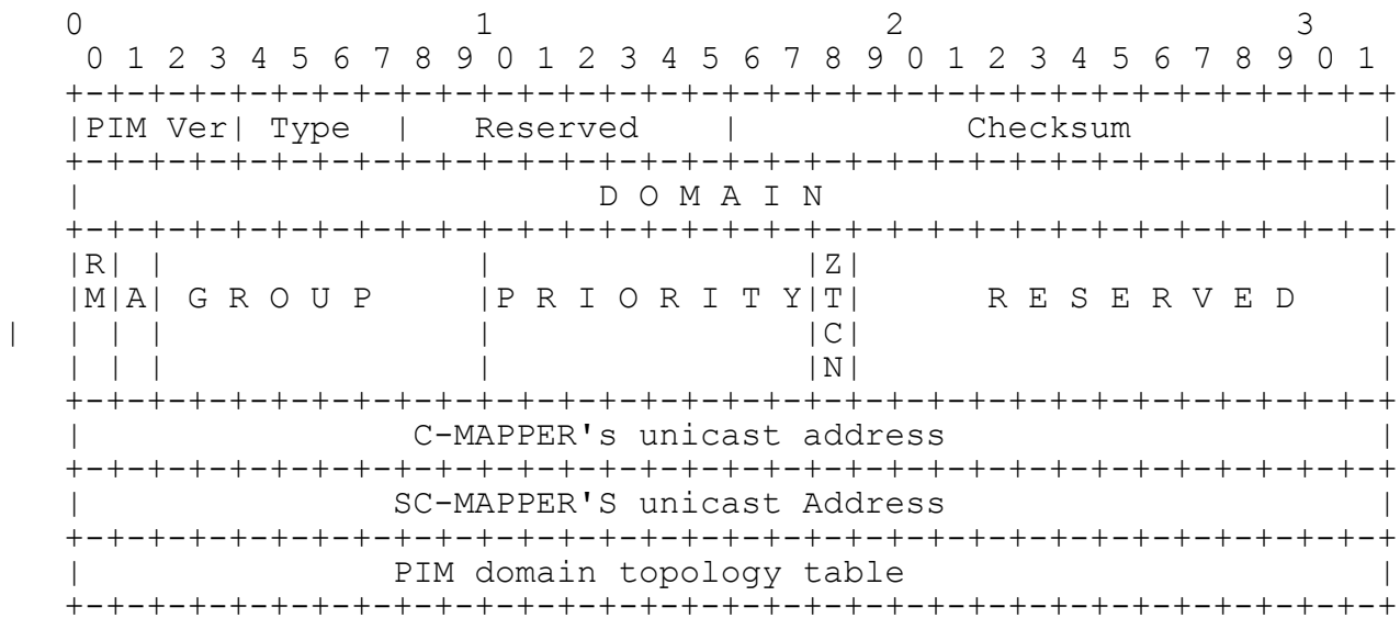
Figure 17 SC-MAPPER/RP answers to a host REQUEST-FOR-C-MAPPER message
