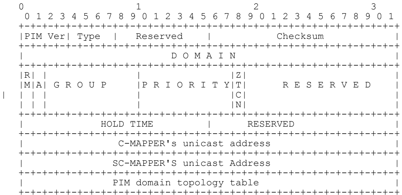
Figure 18 SC-MAPPER/RP multicast introductions to all PIM-NG-CLIENTS
