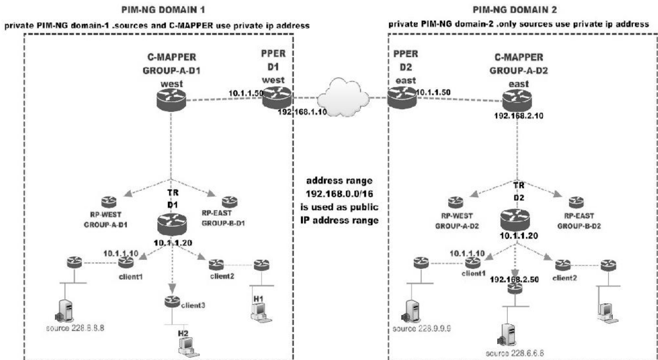
Figure 44 Multicast network with private PIM-NG domains
