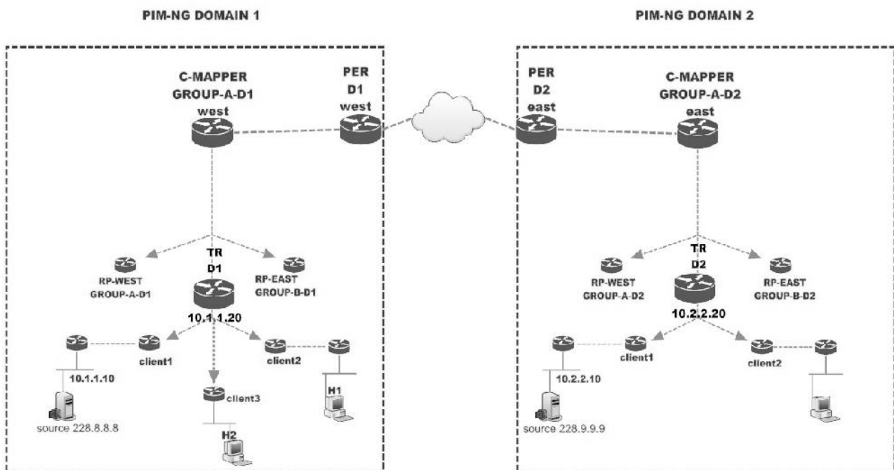
Figure 43 network with 2 multicast domains
