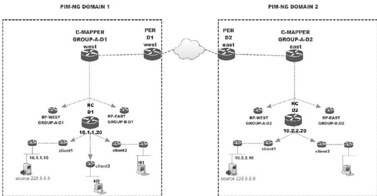
Figure 38 network with 2 PIM-NG multicast domains
