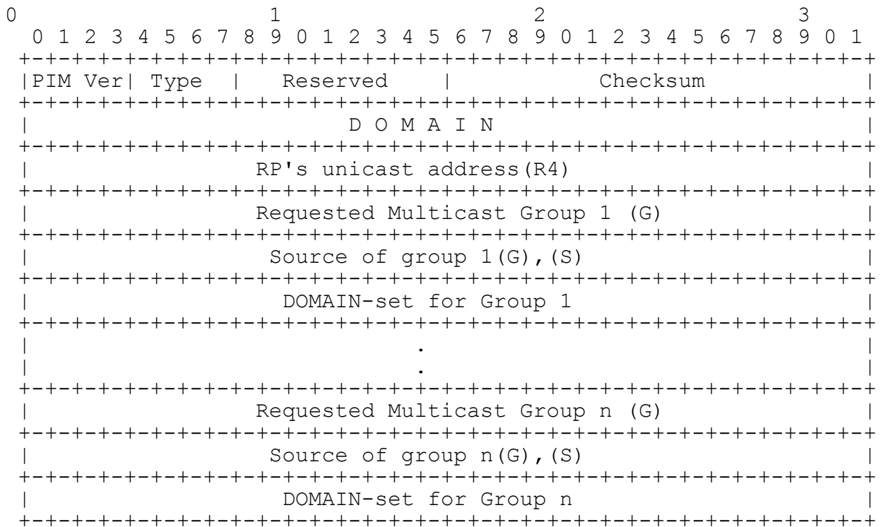
Figure 8 C-RP Acknowledge packet format, sent to the source in case the source exists
