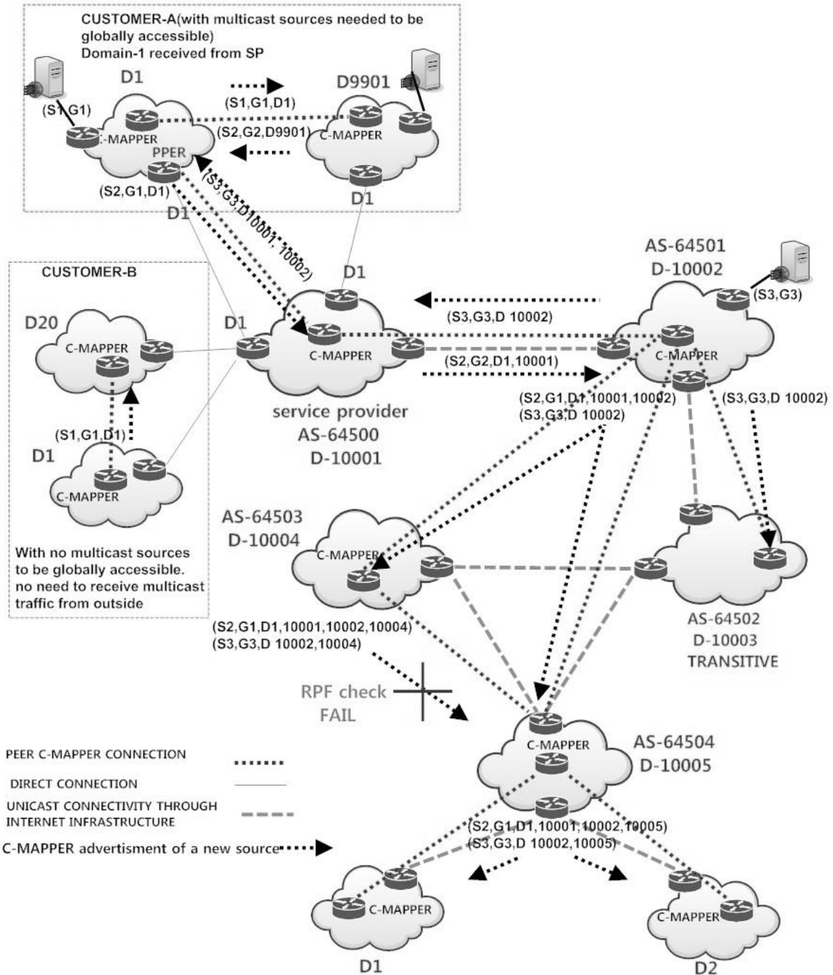
Figure 48 multicast network and multicast advertisements
