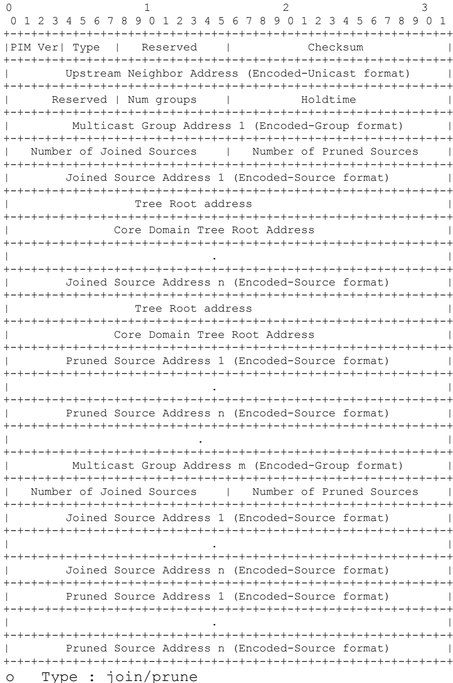
Figure 10 Join/prune message format
