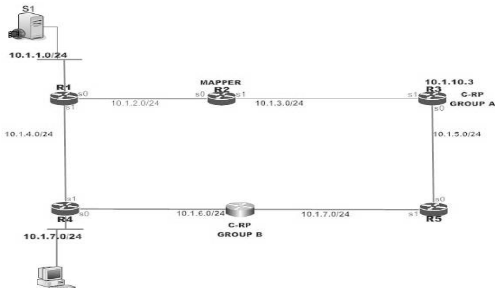
Figure 25 network design with one multicast domain
