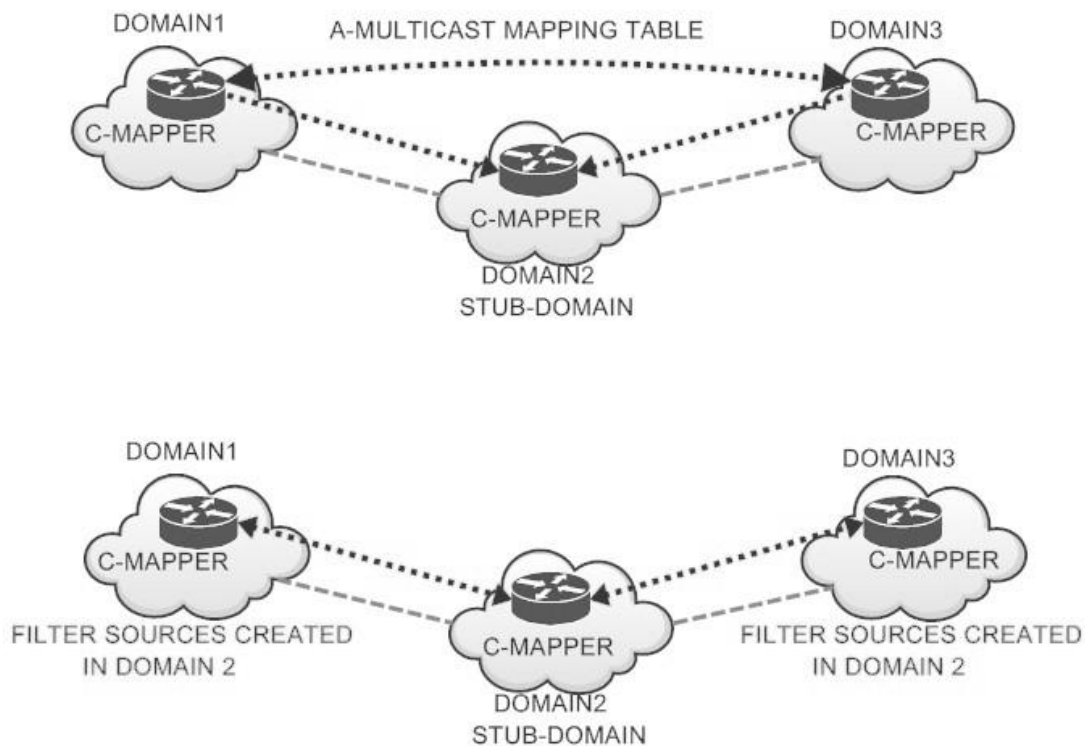
Figure 52 Stub-Domain as the transitory multicast domain
