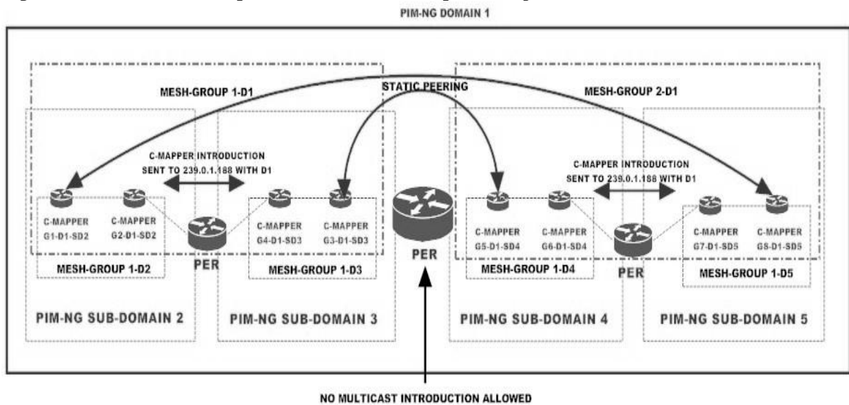
Figure 49 Mesh-Groups and C-MAPPER peering
