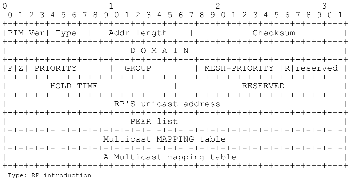
Figure 21 C-MAPPER/RP unicast HELLO/KEEP-ALIVE message to back up RPs
