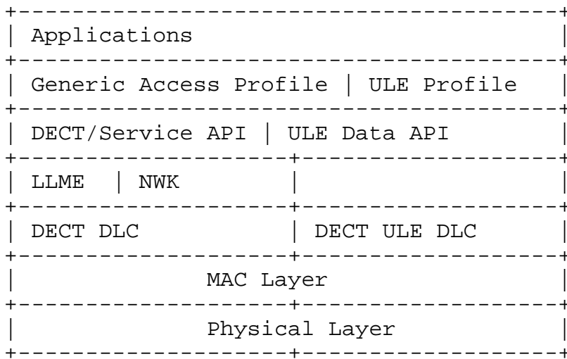
Figure 1: DECT ULE Protocol Stack
