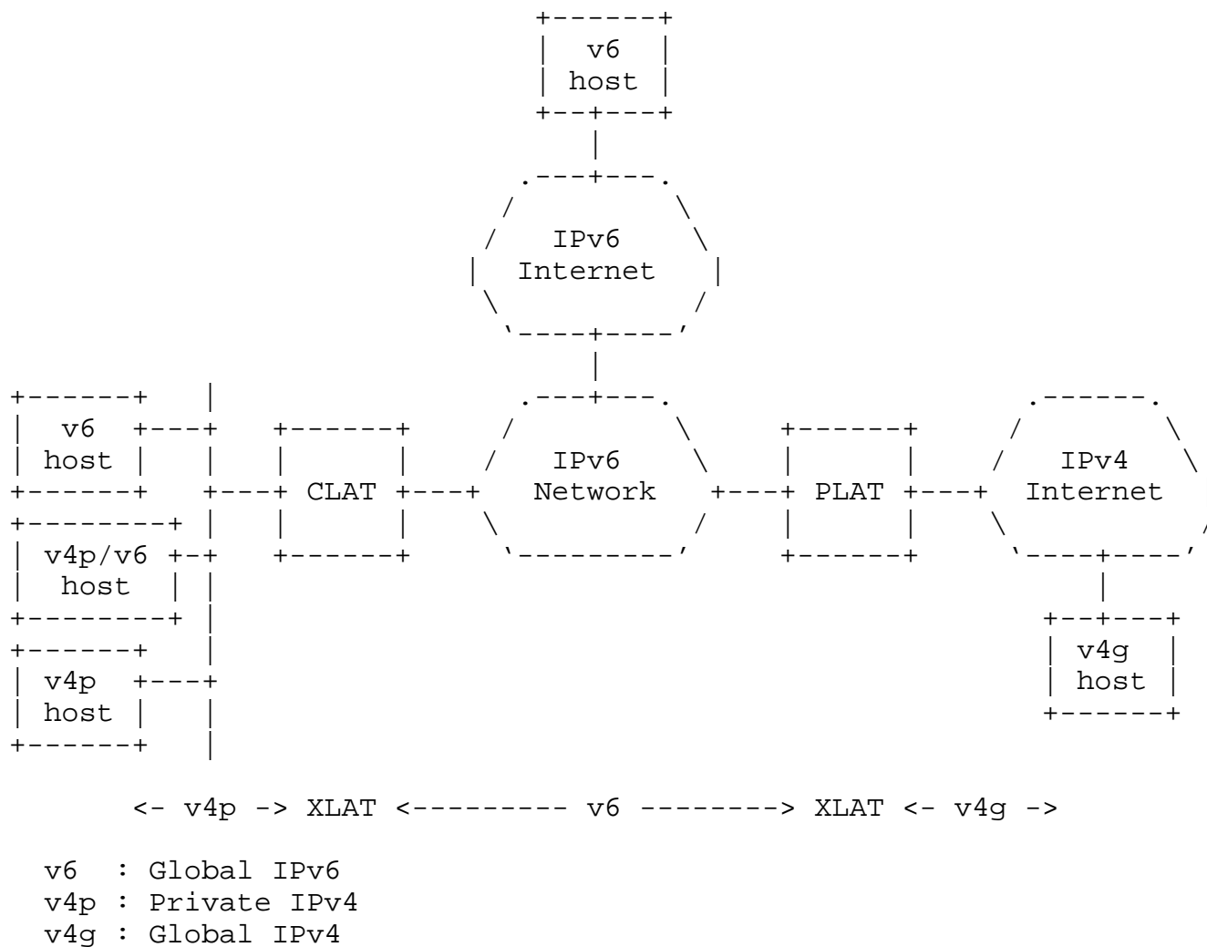
Figure 1: Wireline Network Topology
