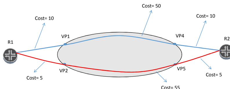
Figure 3 - IP+Optical Path Computation Example
