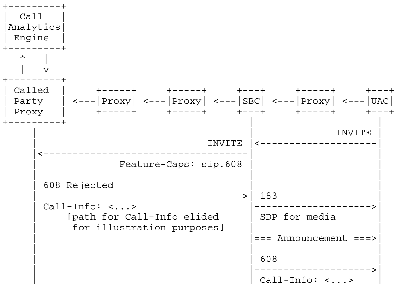
Figure 5: Legacy Operation
