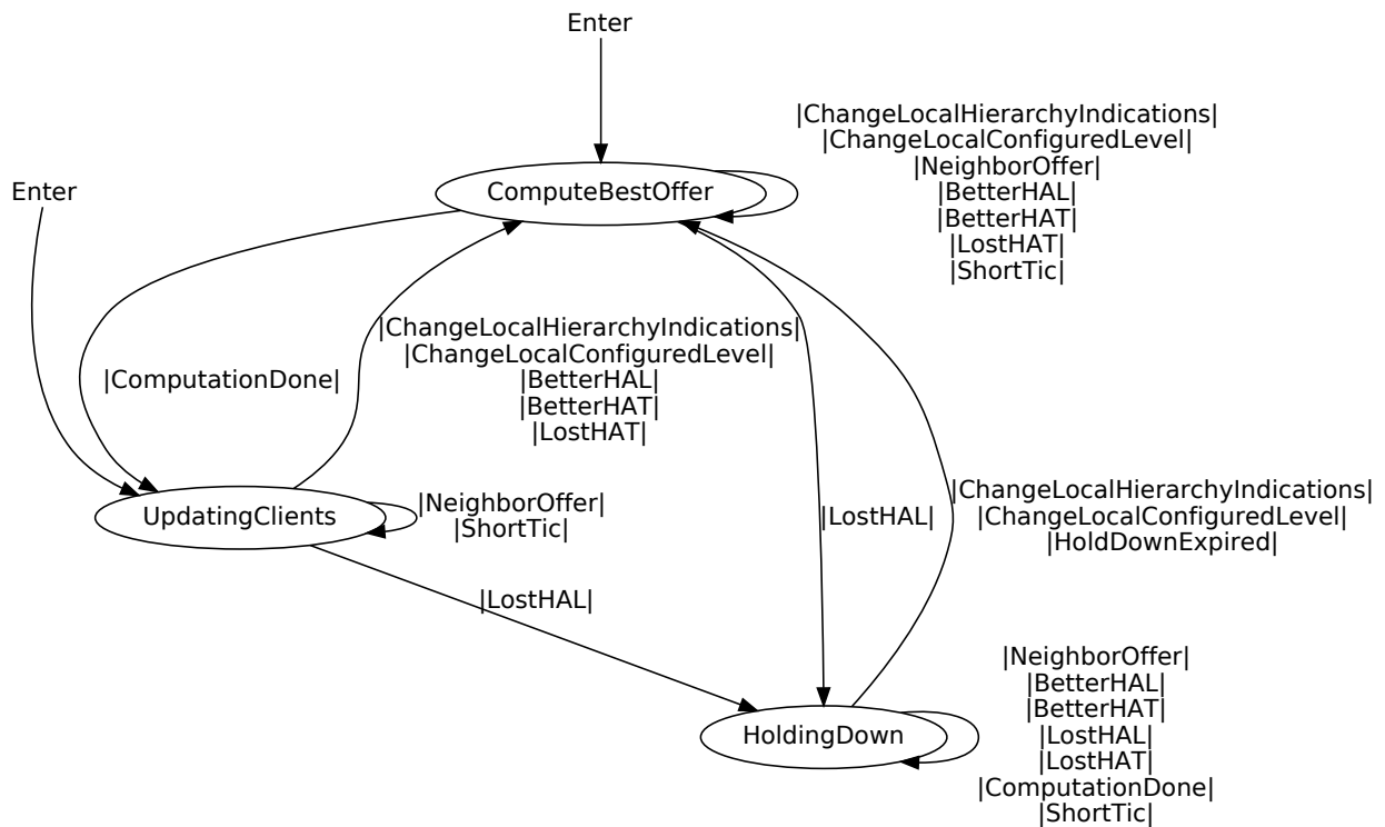
Figure 28: ZTP FSM
