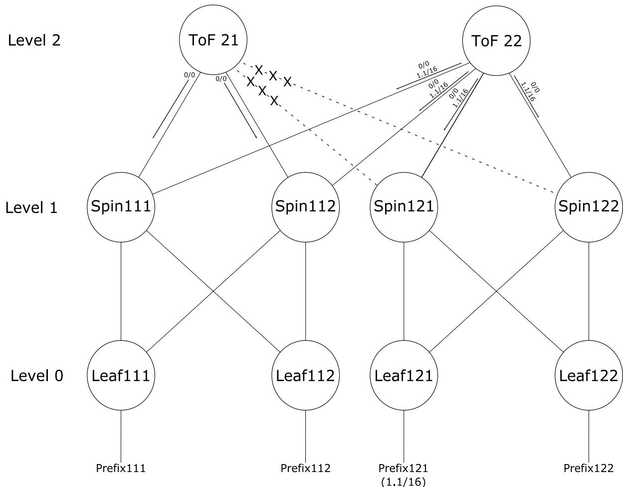
Figure 36: Fabric Partition
