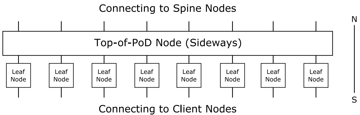
Figure 7: Side View of a PoD, K_{TOP}=8 , K_{LEAF}=6
