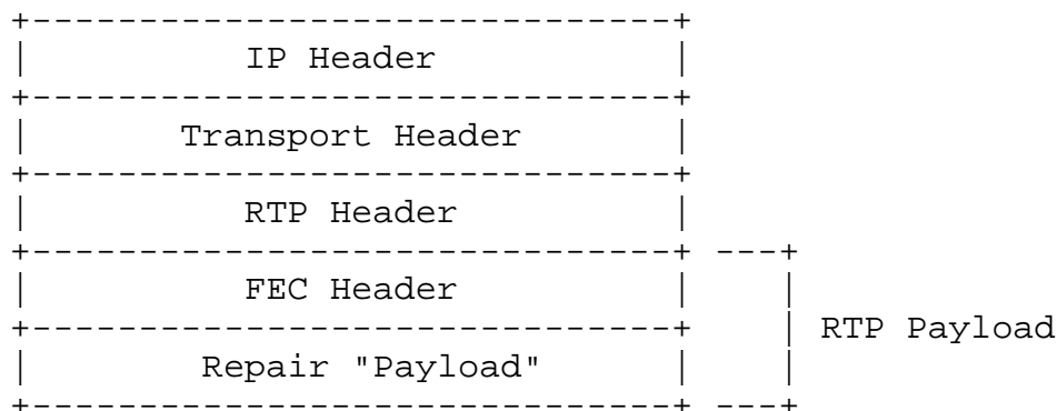
Figure 9: Format of FEC repair packets
