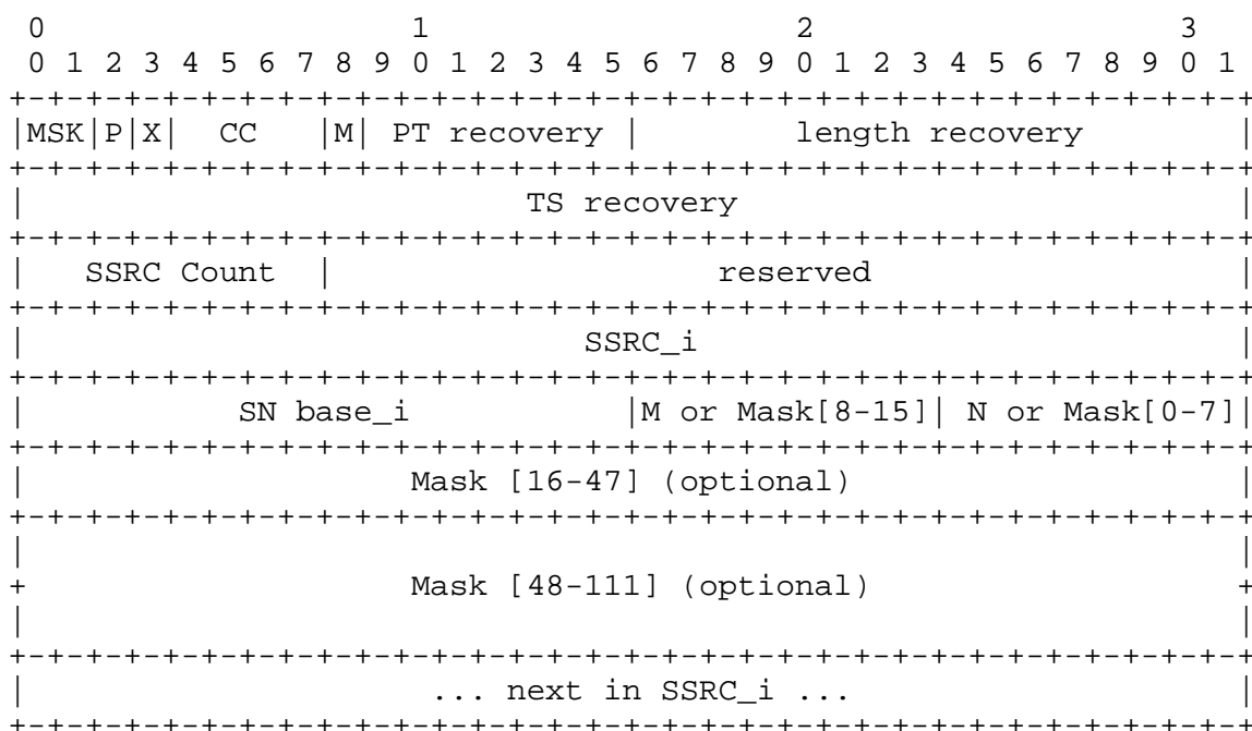
Figure 10: Format of the FEC header
