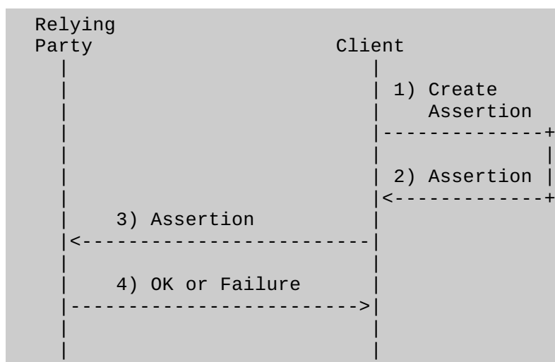
Figure 2: Self-Issued Assertion
