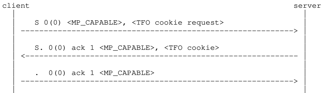
Figure 18: Cookie request
