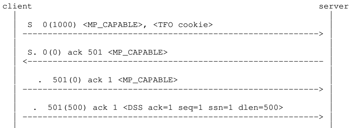
Figure 21: Partial data acknowledgement
