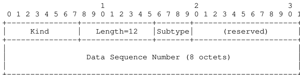
Figure 17: Fallback (MP_FAIL) Option
