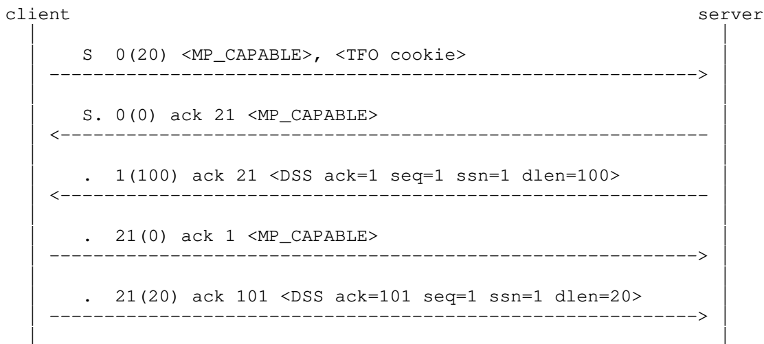
Figure 19: The server supports TFO
