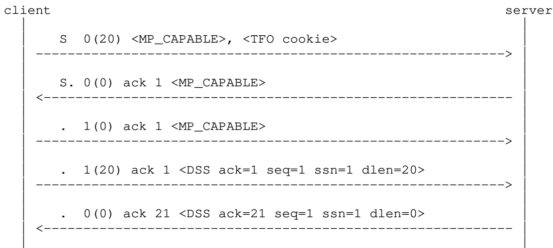
Figure 20: The server does not support TFO
