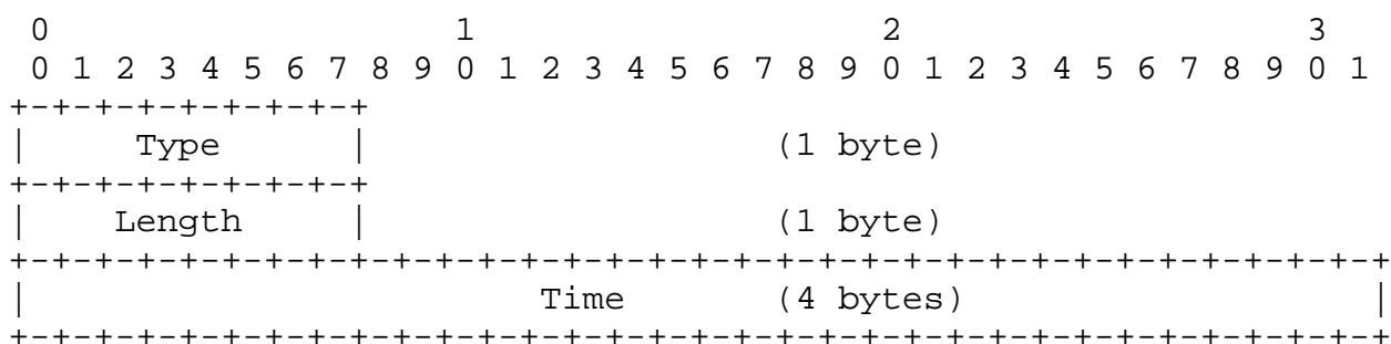
Figure 6: Timestamp sub-TLV
