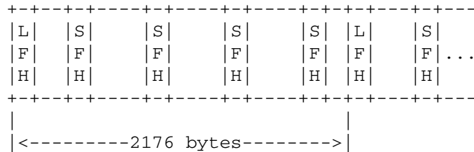
Fig. 14 Example of resynchronization data stream
