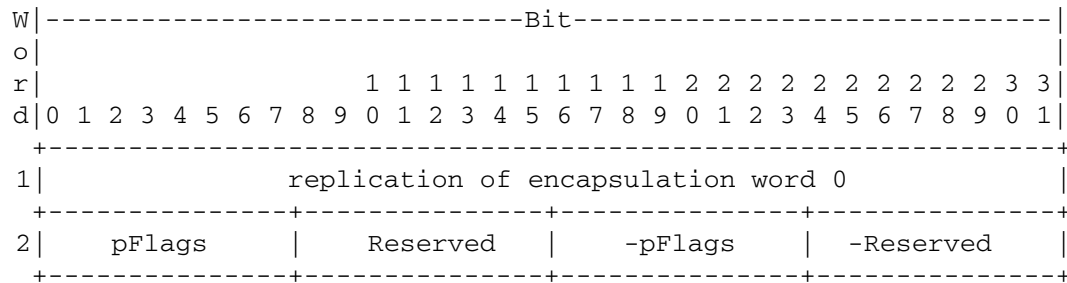
Fig. 7 FCIP Usage of FC Frame Encapsulation Protocol Specific field
