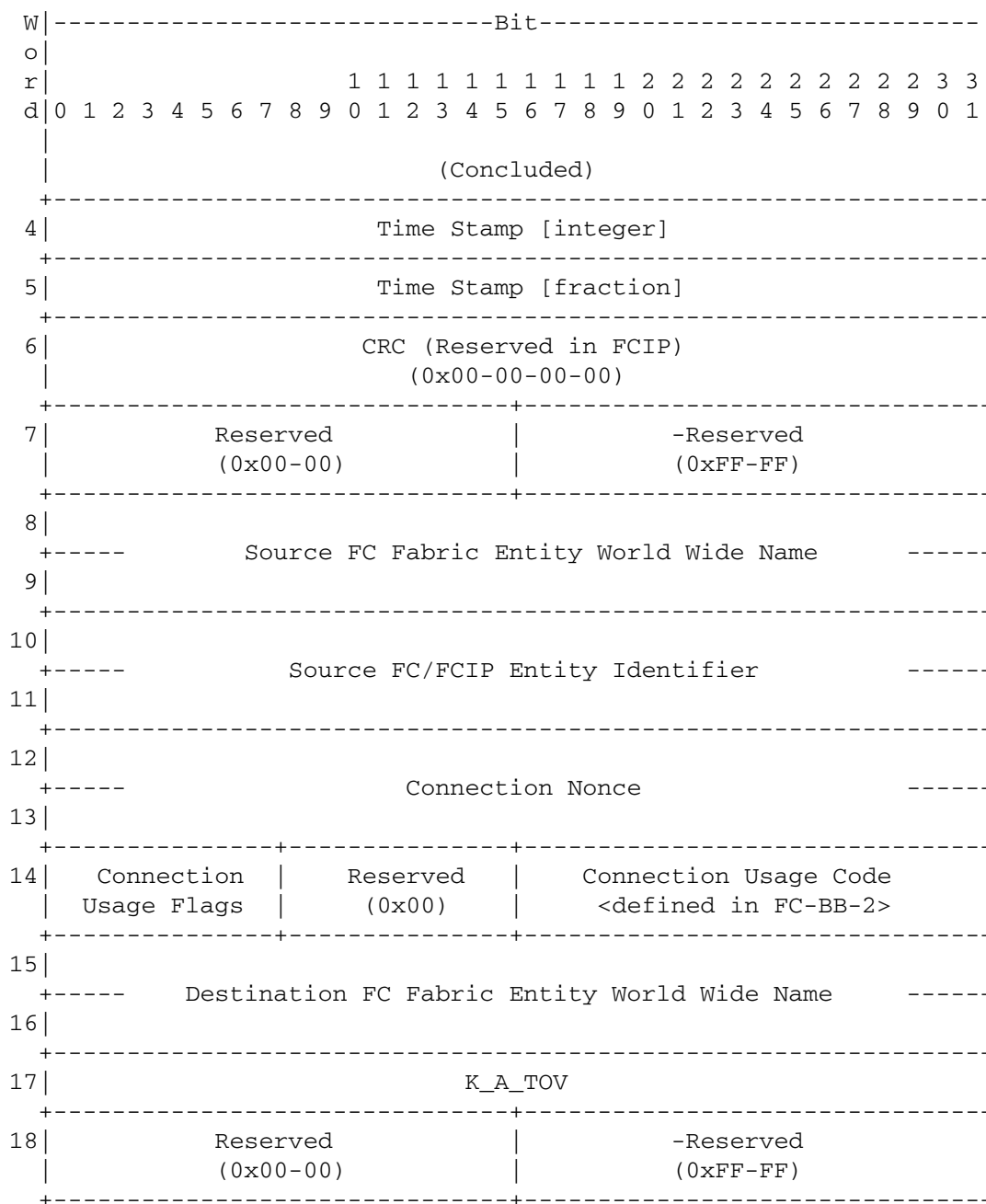
Fig. 9 FSF Format (part 2 of 2)
