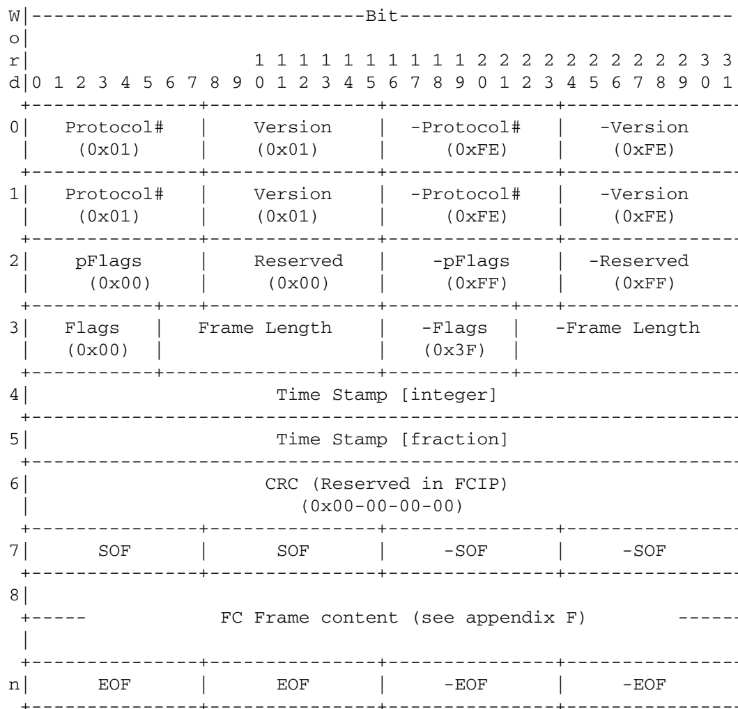
Fig. 17 FCIP Frame Format
