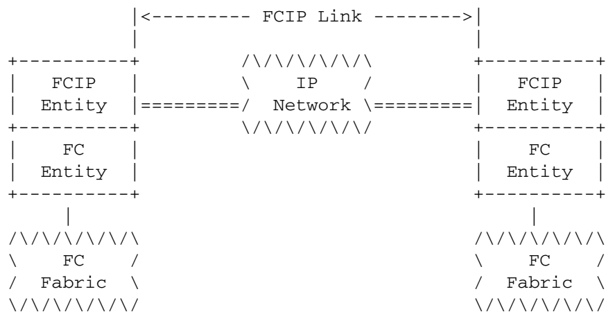
Fig. 3 Model for Two Connected FC/FCIP Entity Pairs
