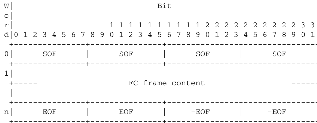
Fig. 5 - FC Frame Encapsulation Format
