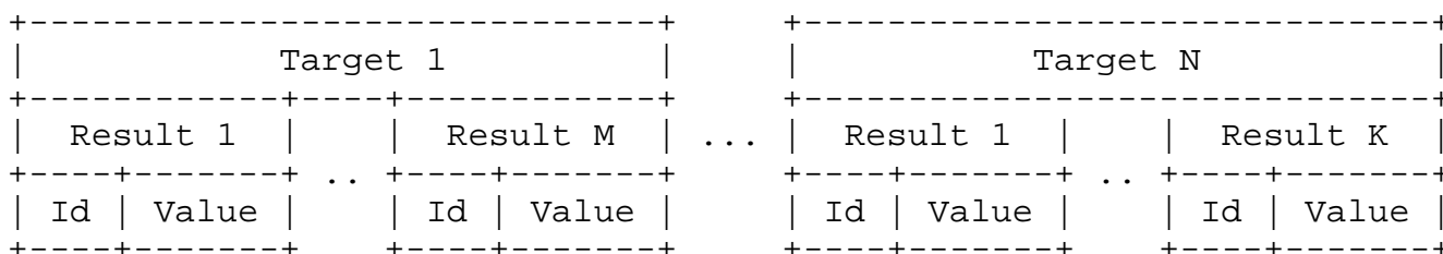
Figure 2: Security Results
