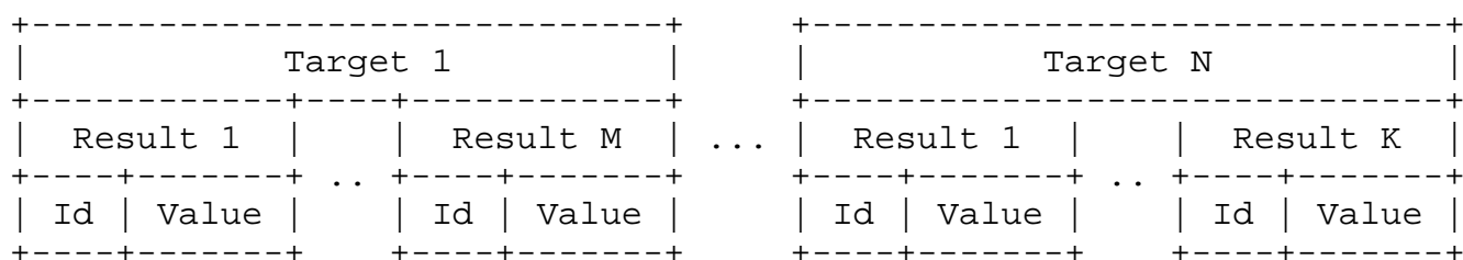
Figure 2: Security Results
