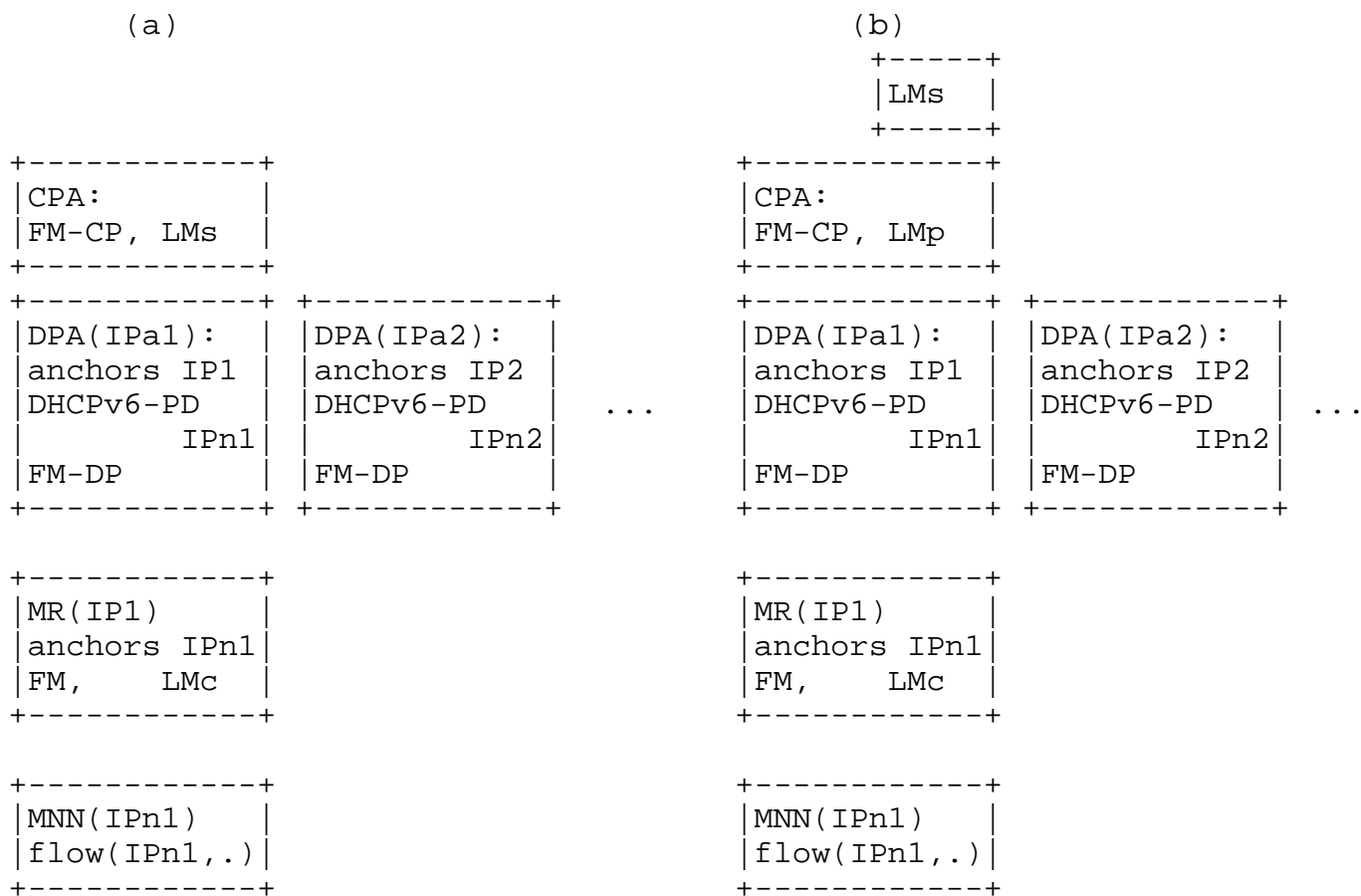
Figure 4. Configurations of NEMO basic support for a MR. (a) FM-CP and LMs at CPA, FM-DP at DPA, FM and LMc at MR; (b) Separate LMs, FM-CP and LMp at CPA, FM-DP at DPA, FM and LMc at MR.
