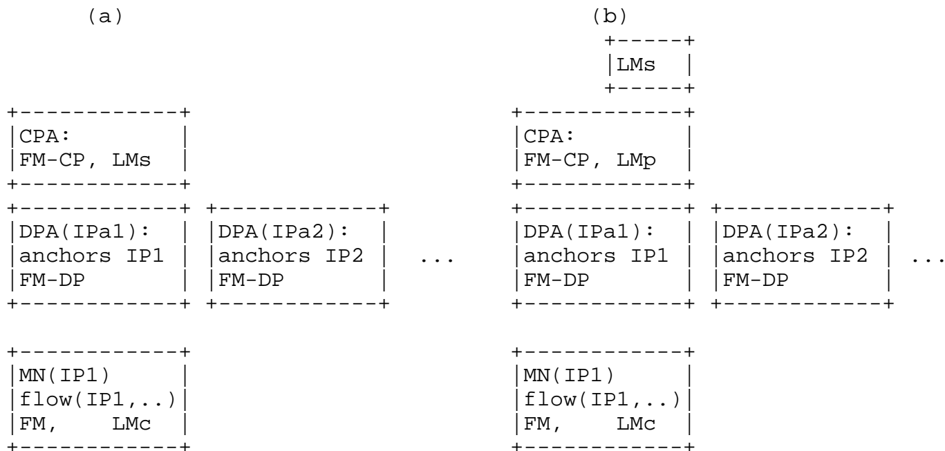
Figure 3. Configurations of host-based mobility management (a) FM-CP and LMs at CPA, FM-DP at DPA, FM and LMc at MN; (b) Separate LMs, FM-CP and LMp at CPA, FM-DP at DPA, FM and LMc at MN.
