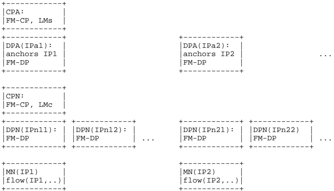
Figure 2(a). Configurations of network-based mobility management for a hierarchical network with FM-CP and LMs at CPA, FM-DP at DPA; FM-CP and LMc at CPN, FM-DP at DPN.
