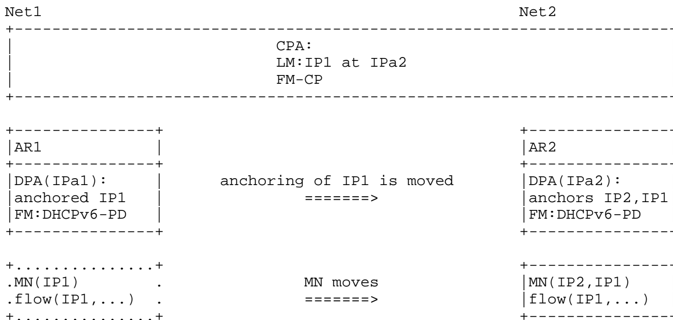
Figure 9. IP prefix/address anchor switching to the new network with the LM and the FM-CP in a centralized control plane whereas the FM-DPs are distributed.
