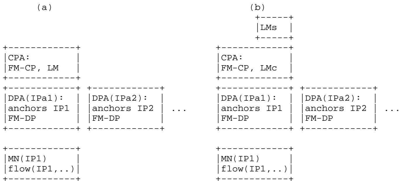
Figure 1. Configurations of network-based mobility management for a flat network (a) FM-CP and LM at CPA, FM-DP at DPA; (b) Separate LMs, FM-CP and LMc at CPA, FM-DP at DPA.
