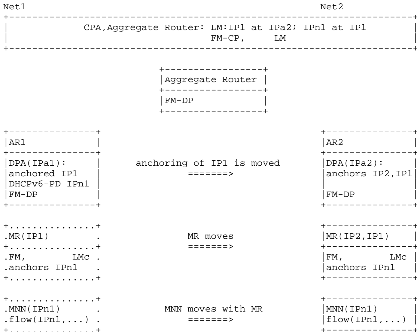
Figure 13. Mobility involving change of IP anchoring for a MR to which an MNN is attached.
