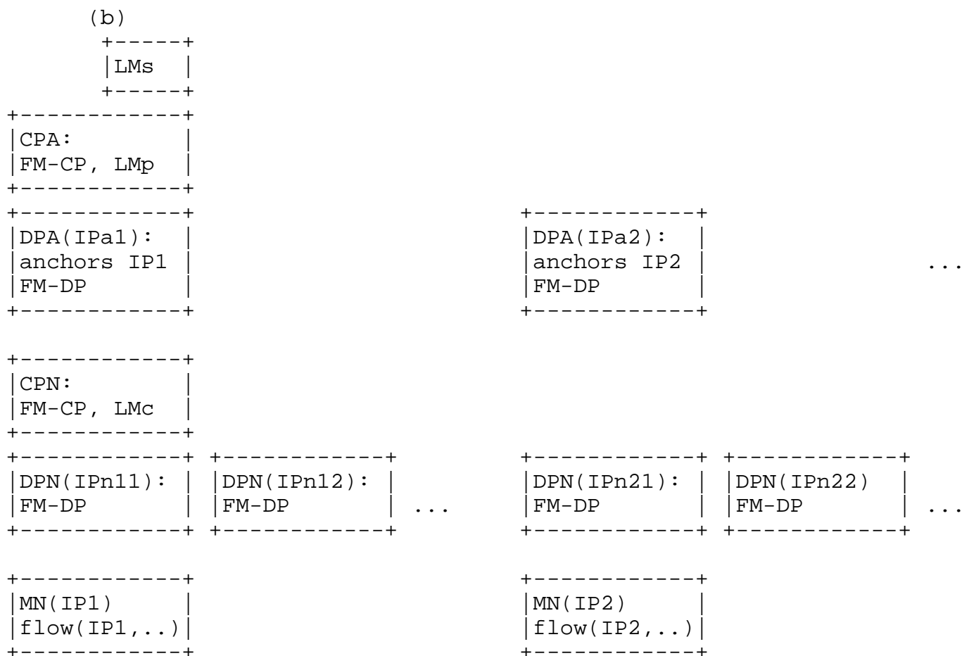
Figure 2(b). Configurations of network-based mobility management for a hierarchical network with separate LMs, FM-CP and LMp at CPA, FM-DP at DPA; FM-CP and LMc at CPN, FM-DP at DPN.
