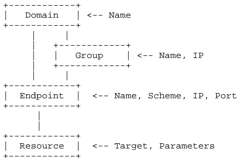
Figure 2: The resource directory information hierarchy.
