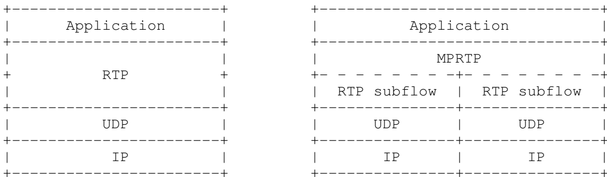
Figure 2: MPRTTP Architecture
