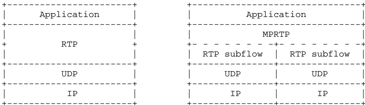
Figure 2: MPRTTP Architecture
