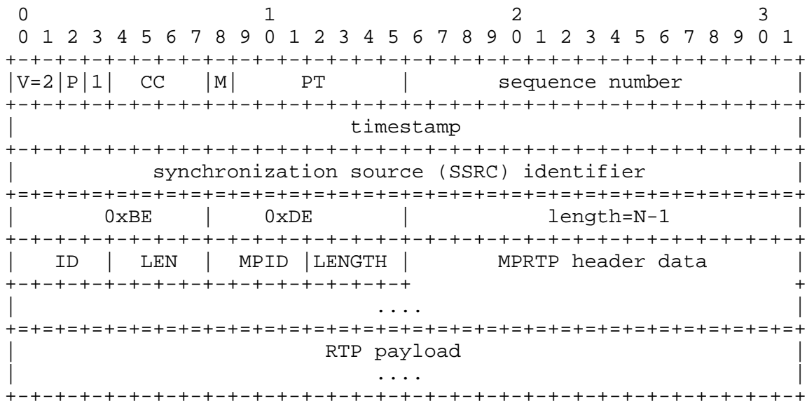
Figure 6: Generic MPRTTP header extension
