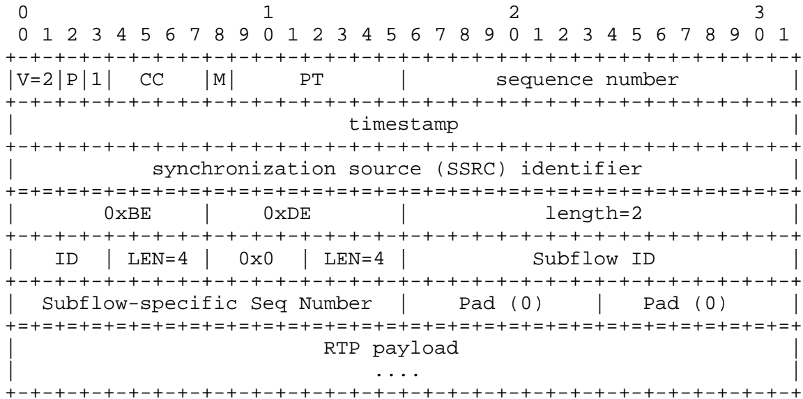
Figure 8: MPRTTP header for subflow
