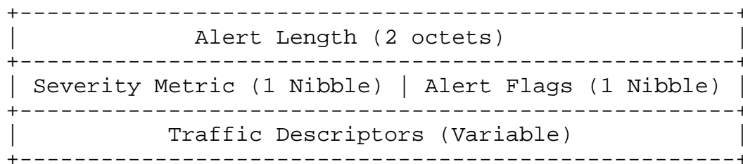
Figure 1: DDoS-AE Alert Attribute
