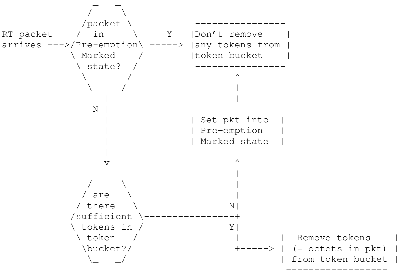
Figure 4: Router action to support explicit pre-emption alerting
