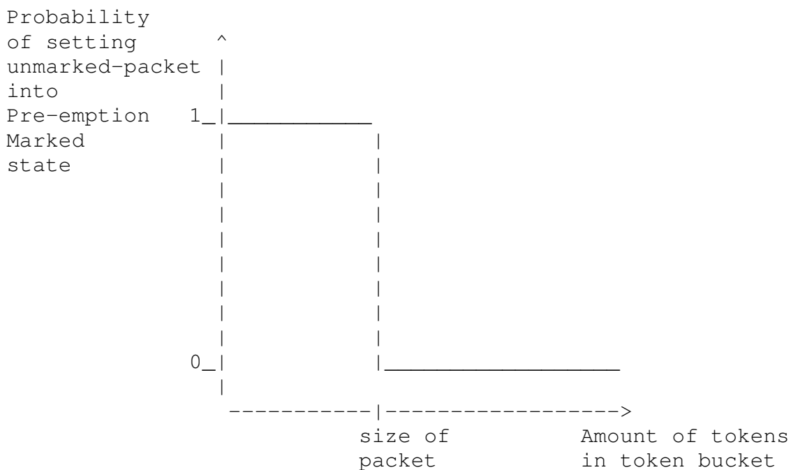
Figure 5: Probability of router setting a packet into Pre-emption Marked state
