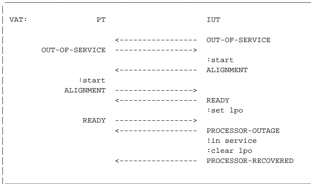
Figure 3.1.15-2. Set and clear LPO when "Aligned ready"
