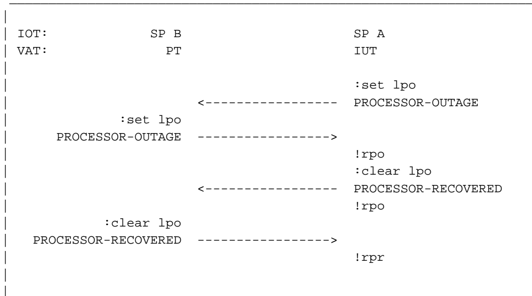
Figure 3.4.3-1. Clear LPO when "Both processor outage"
