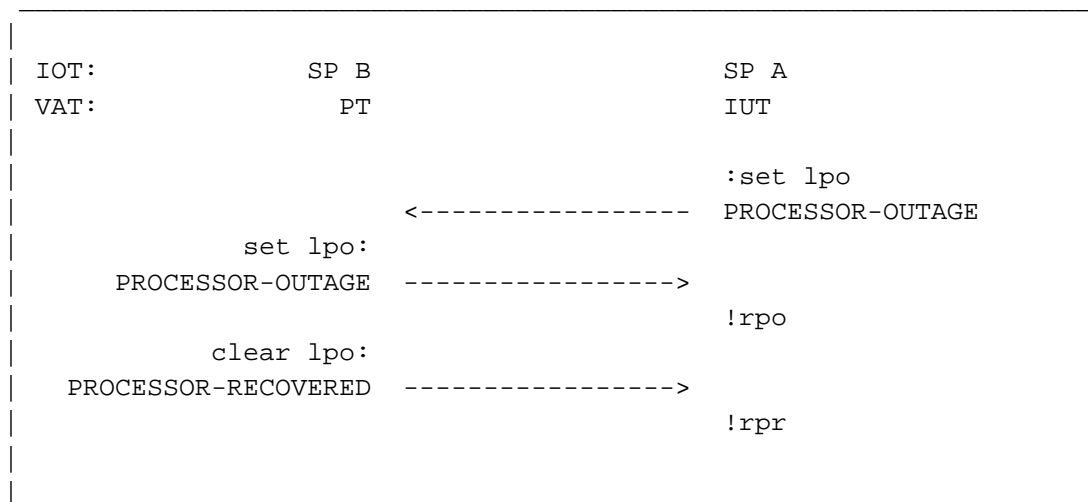
Figure 3.4.2-1. RPO during LPO
