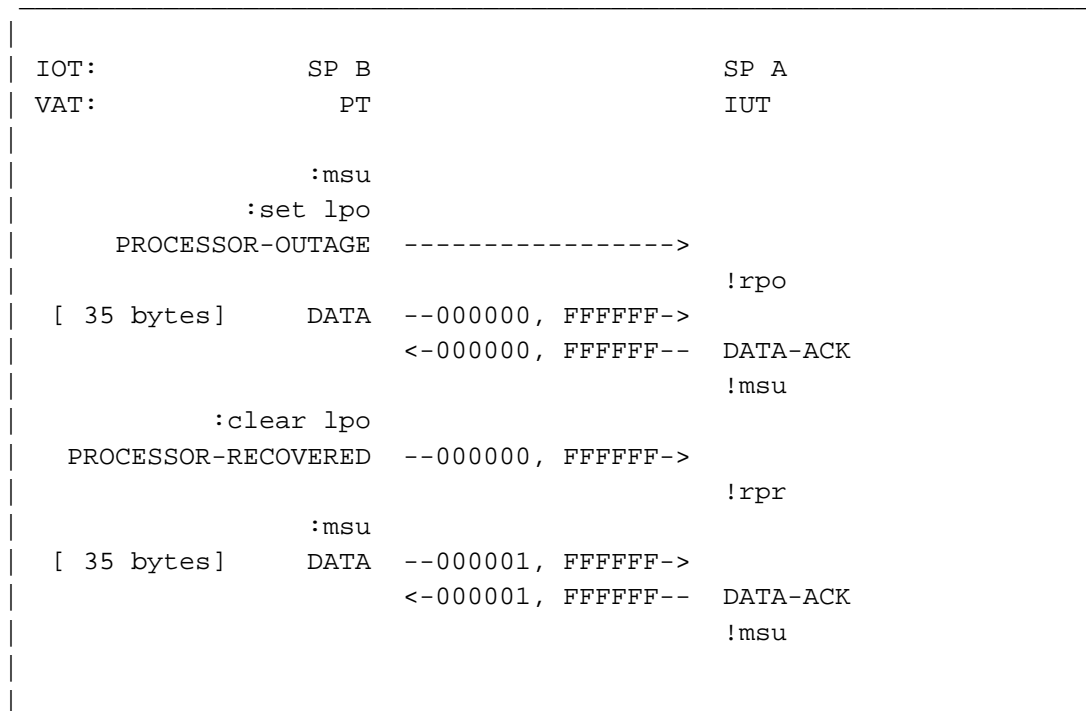
Figure 3.8.9-1. In service prior to RPO being set
