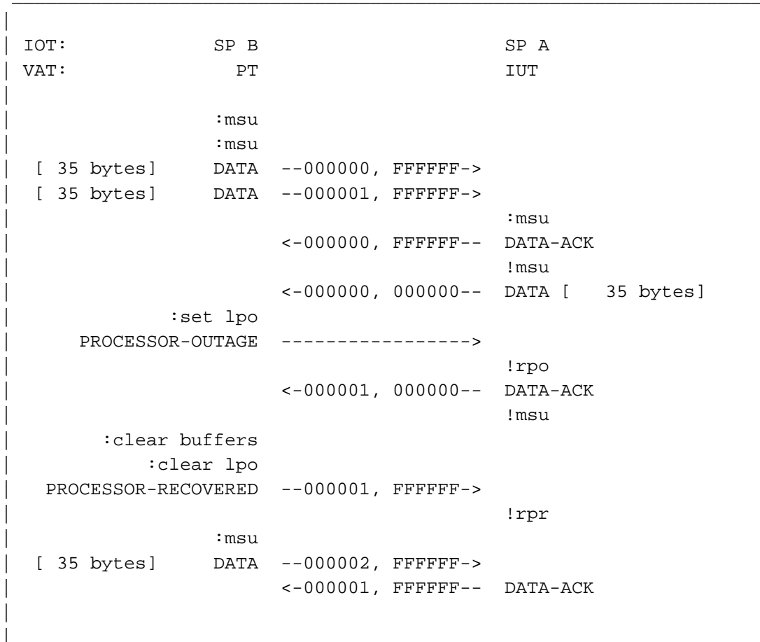
Figure 3.4.1-2. Set and clear RPO while link in service
