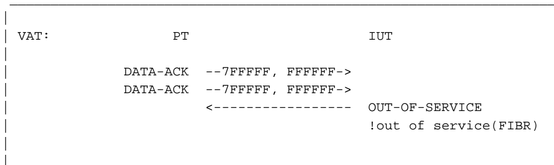
Figure 3.3.2-1. Link aligned ready (Invalid Acks)
