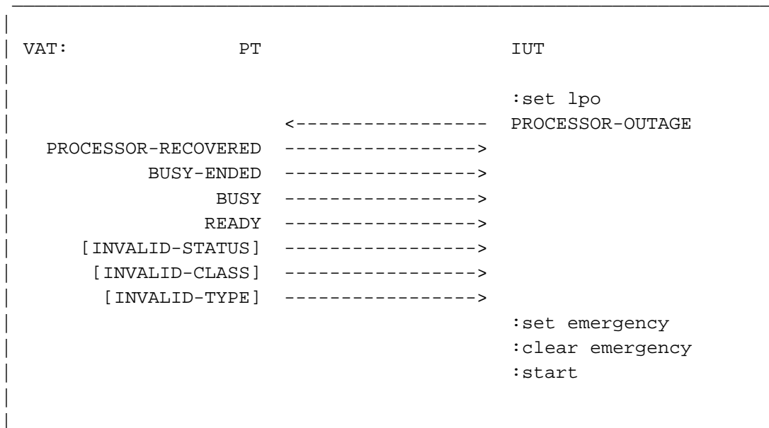
Figure 3.2.8-1. Unexpected events while "processor outage"
