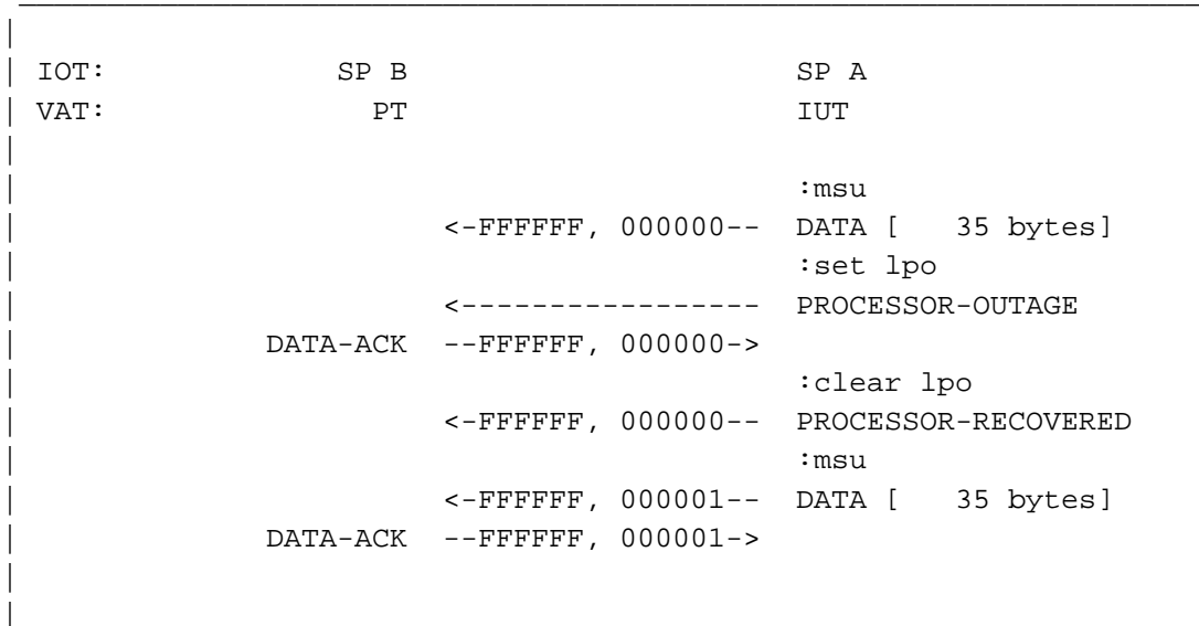
Figure 3.8.9-2. In service prior to RPO being set
