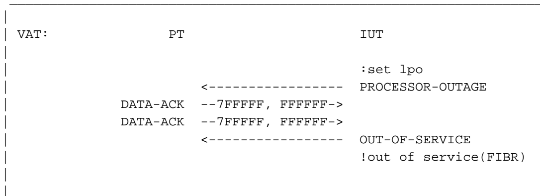
Figure 3.3.8-1. Link in processor outage (Invalid Acks)
